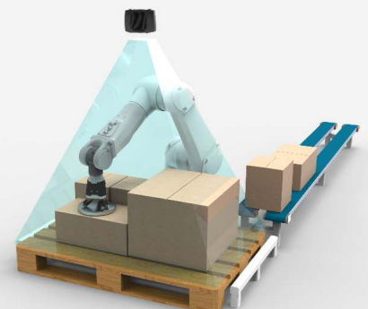
Depalletizing Mono-Caméra
